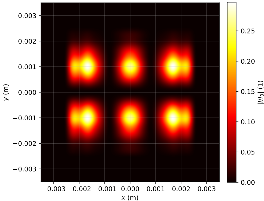
Intensity profile I(x, y, z = 3.981)/I_0 , \text{Pin}=2.0\text{Pcr} , artificial time
